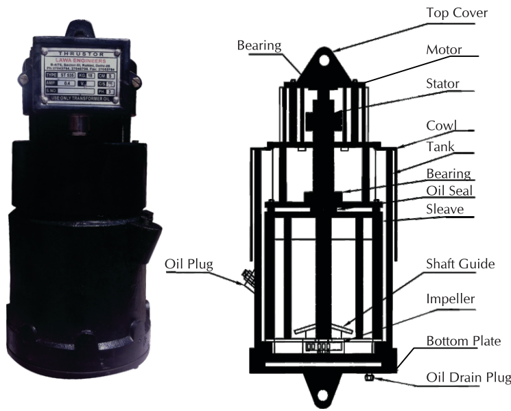
THRUSTOR ST-520
