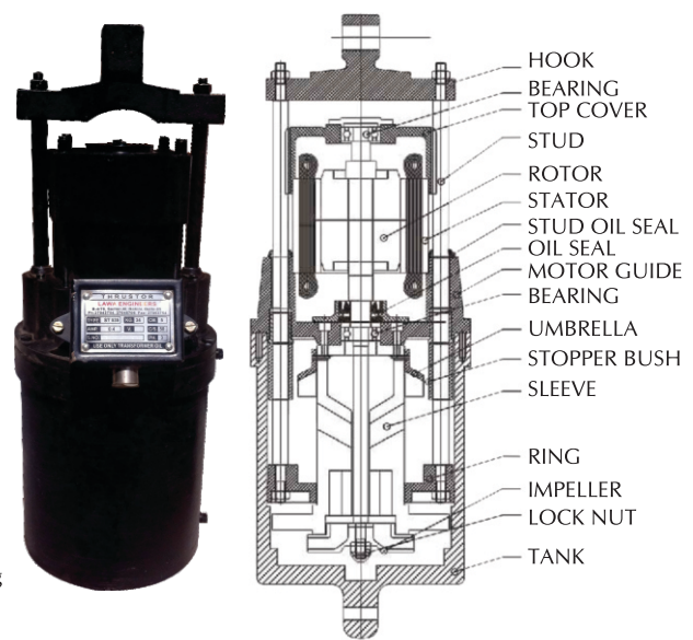
THRUSTOR ST-535
