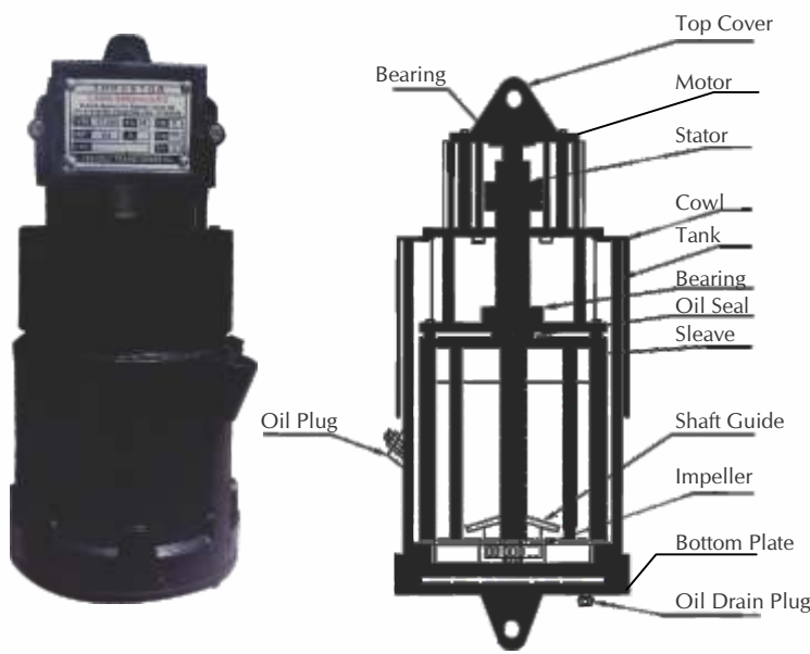
THRUSTOR ST-520
